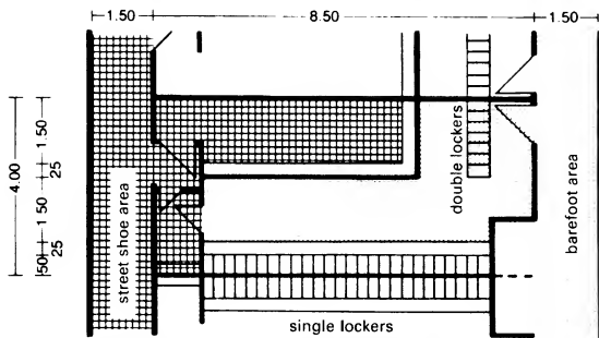
③ Communal changing with supplementary bench
